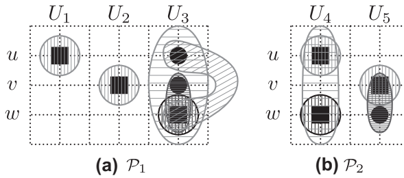
Figure 3. Non-trivial sets in different structures.
