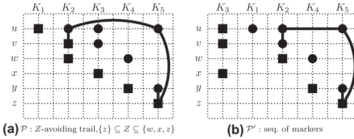
Figure 2. Sequence of markers in structure (K_1, \dots, K_5) and its reordering.
