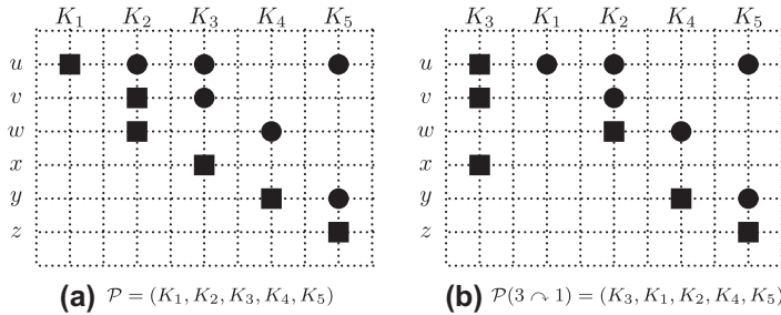
Figure 1. Persegram of structure (K_1, \dots, K_5) and its reordering.
